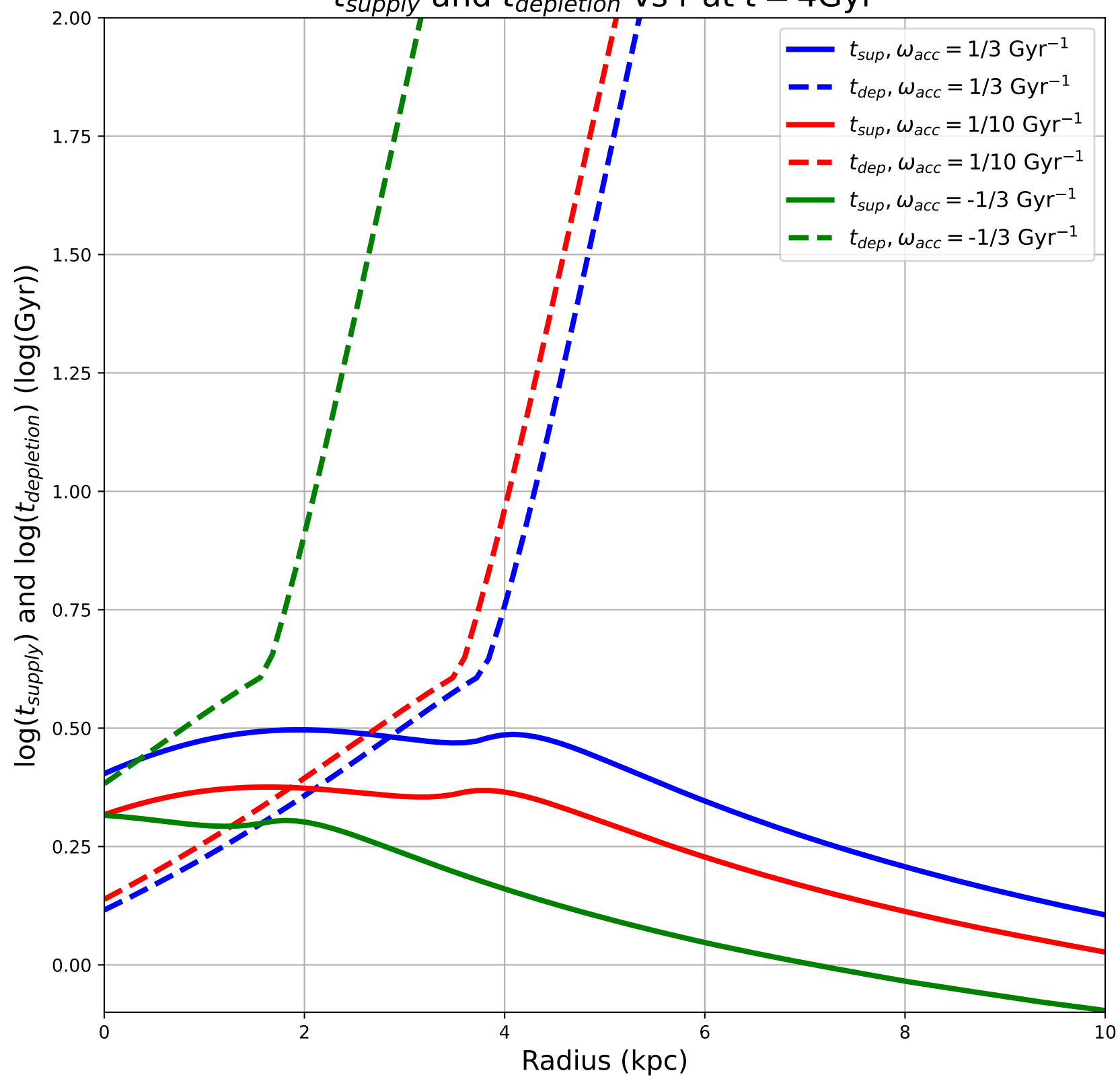
t_{supply} and t_{depletion} vs r at t = 4\text{Gyr}
